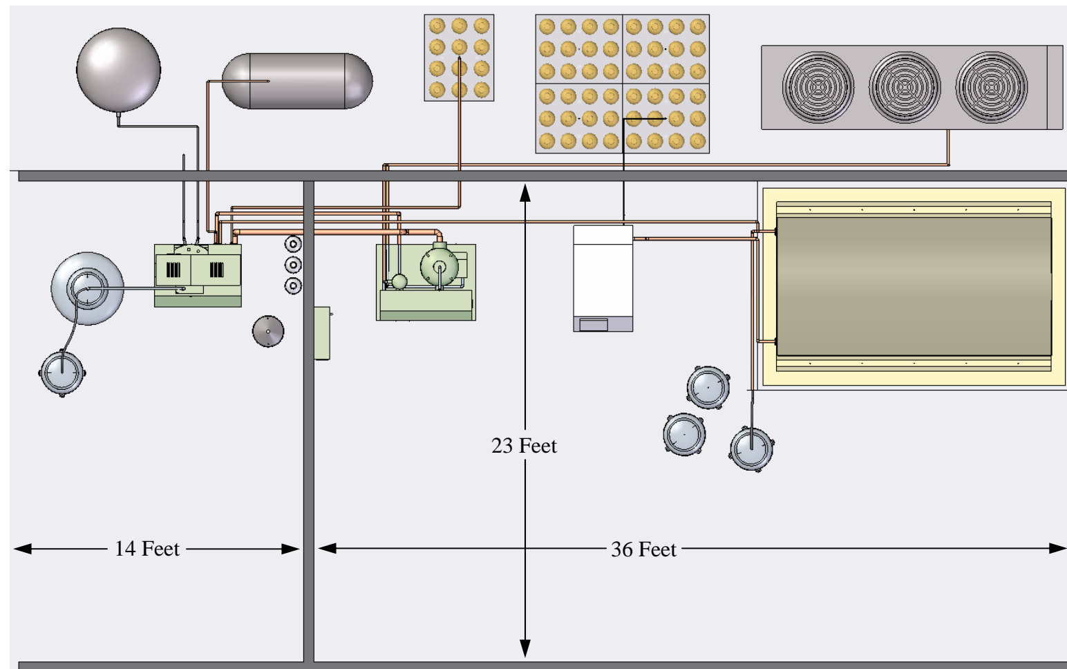
Top Dimensional View
